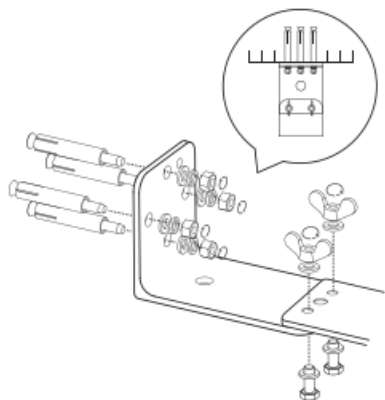
Figure 1: Mounting bracket (wall bracket) and anchor dowels provided. Connection from the wall to the infrared heater.
